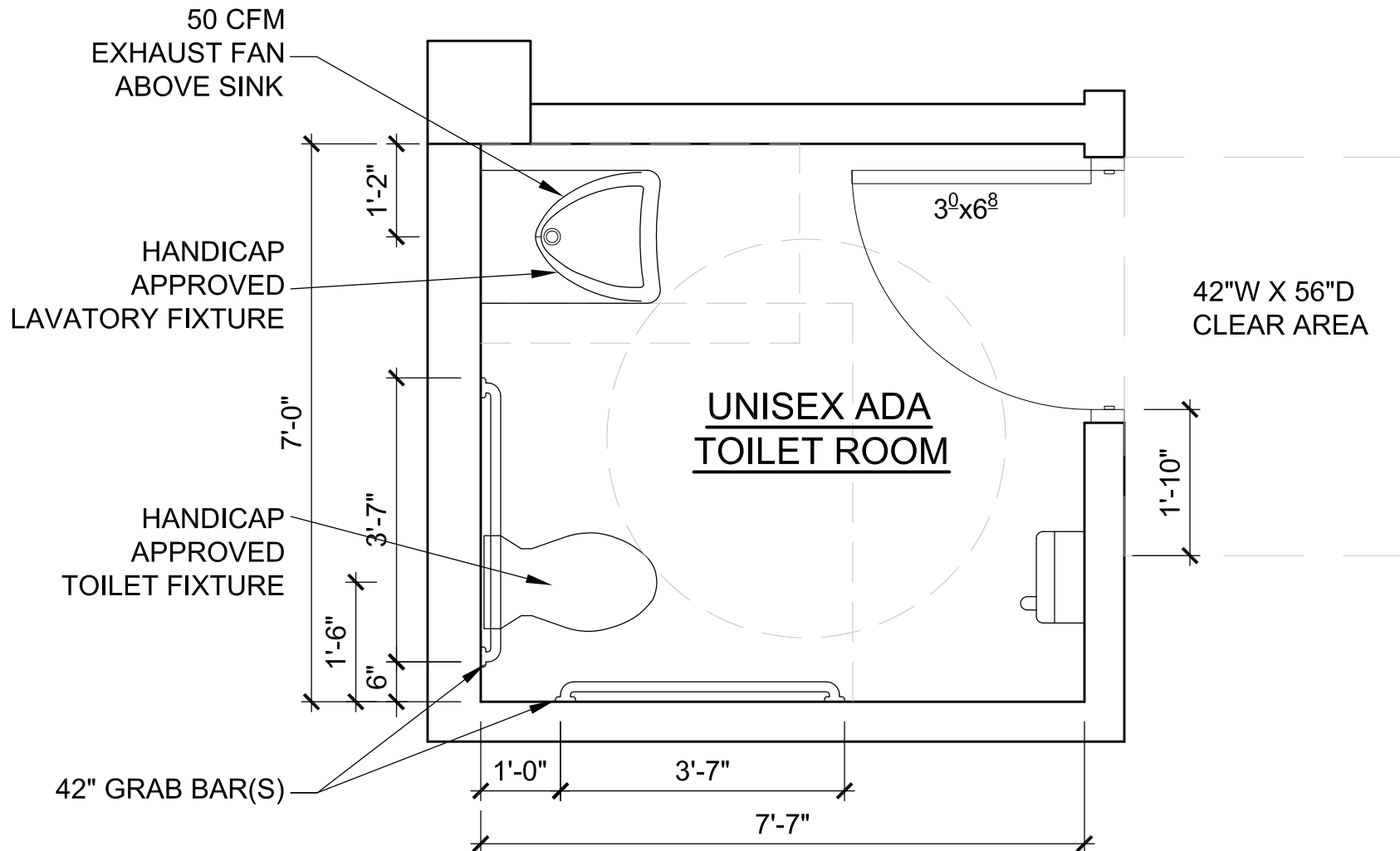
1 TYPICAL ENLARGED ADA TOILET ROOM NOT TO SCALE
