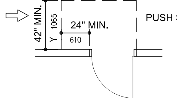
LATCH SIDE APPROACHES - SWINGING DOORS
