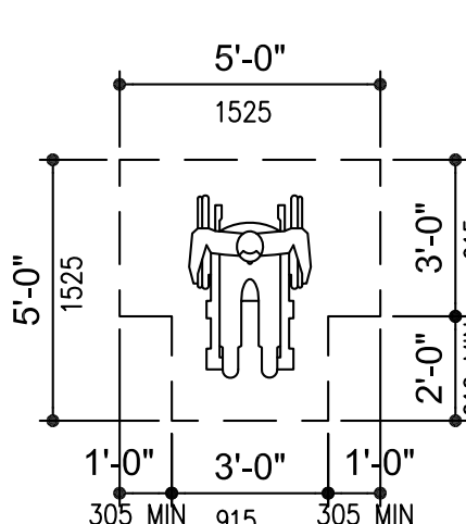
T-SHAPED TURNING SPACE
