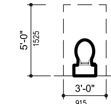
CLEAR FLOOR SPACE AT TOILETS
