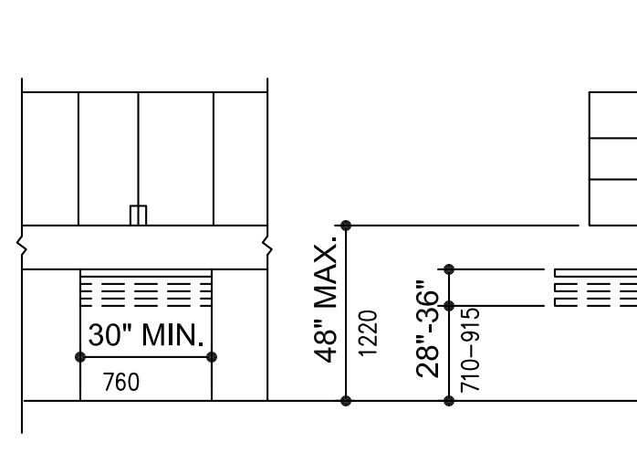
CABINETS AND BASE REMOVED AND HEIGHT ALTERNIVES
