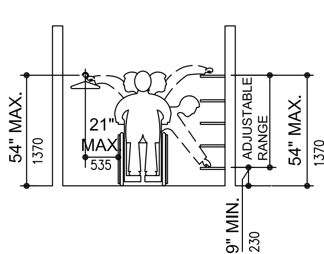
STORAGE SHELVES AND CLOSETS
