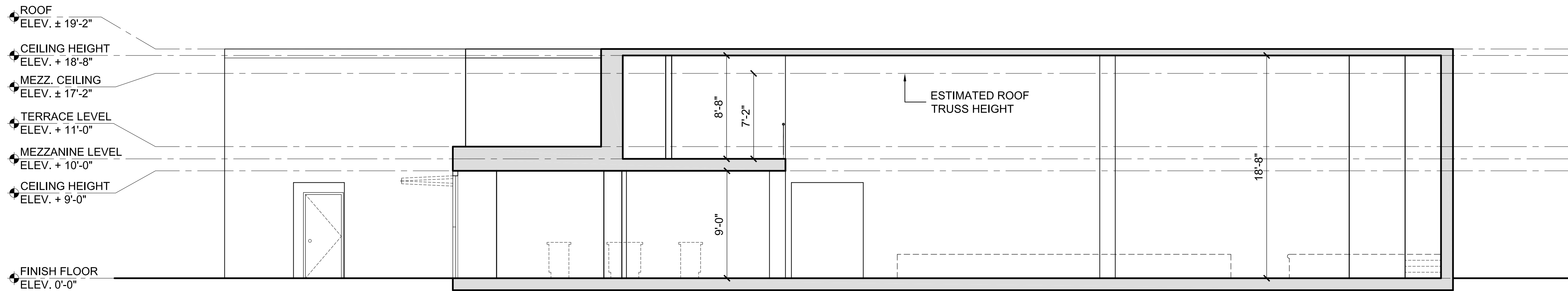
1 PROPOSED SECTION SCALE: 3/16" = 1'-0"
