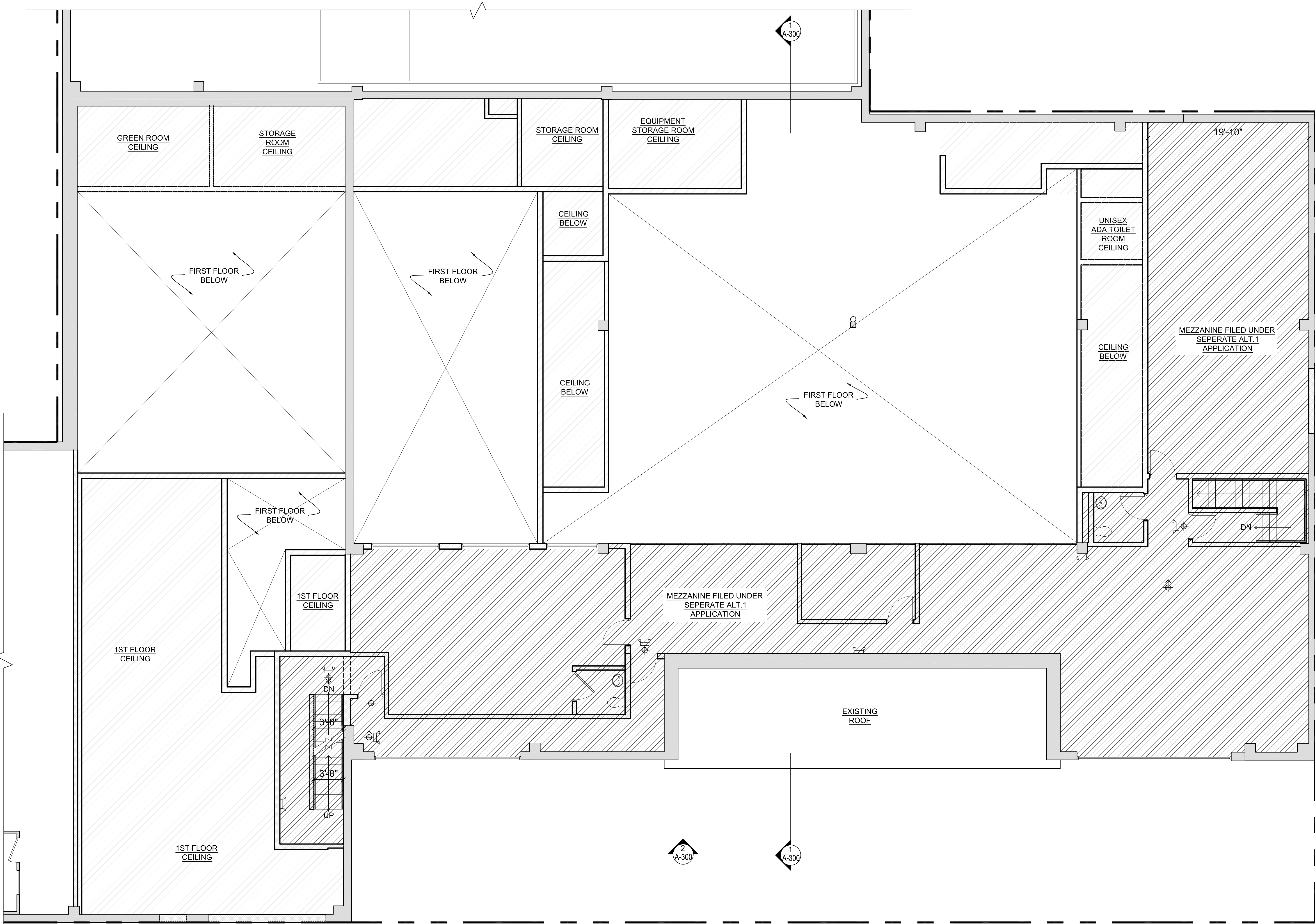
1 PROPOSED MEZZANINE PLAN SCALE: 3/16" = 1'-0"
