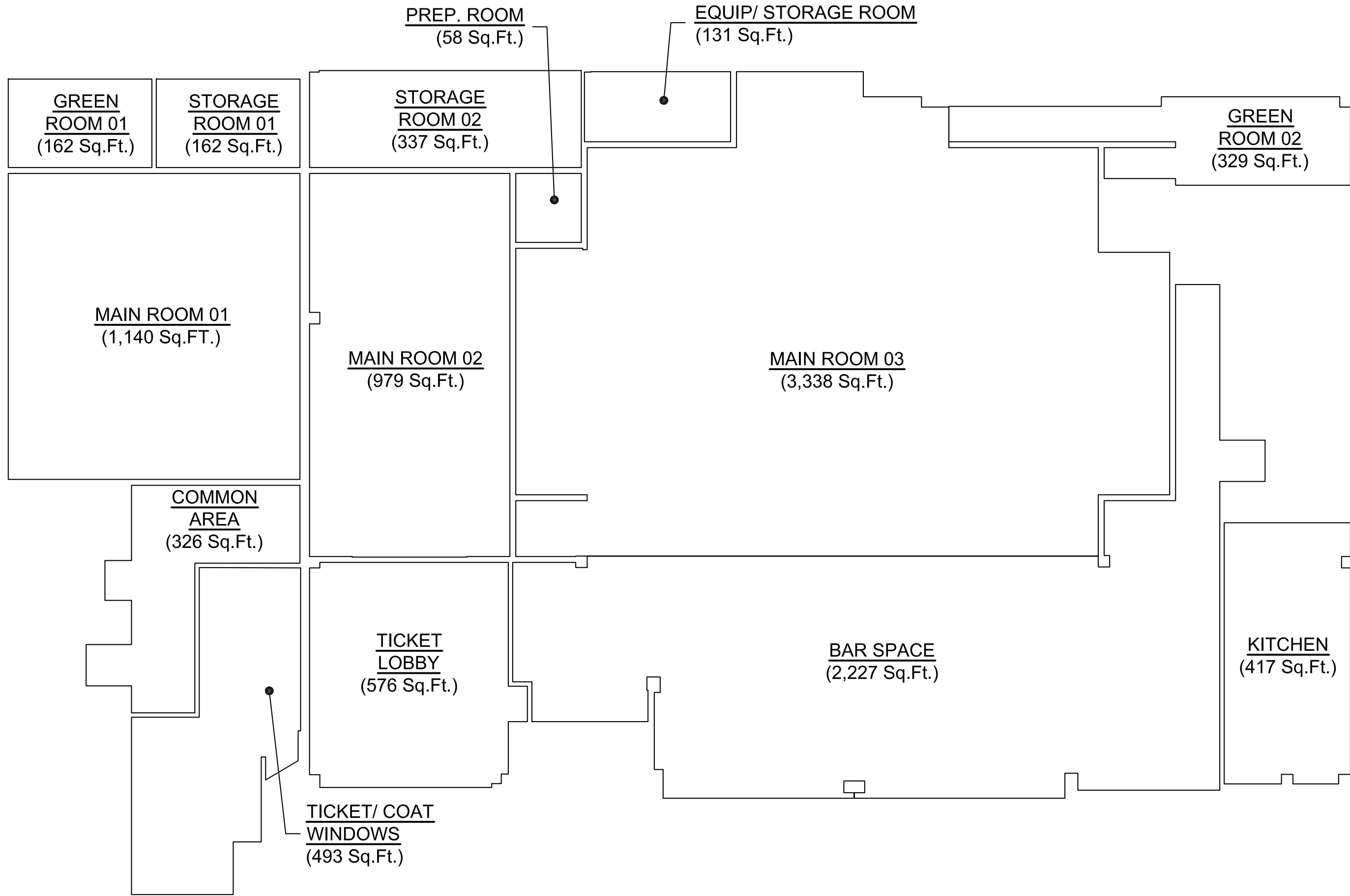
1 PROPOSED 1ST FLOOR PLAN SCALE: 3/32" = 1'-0"
