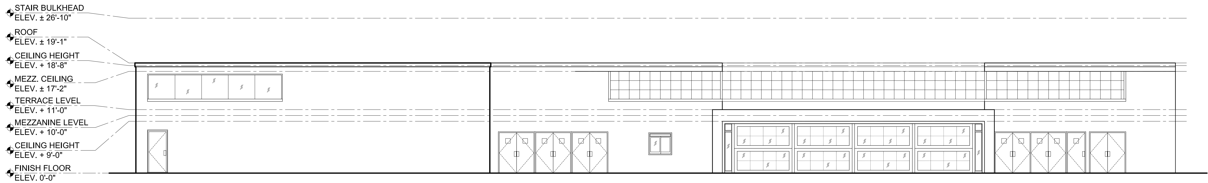
2 PROPOSED ELEVATION - RANDOLPH STREET SCALE: 1/8" = 1'-0"
