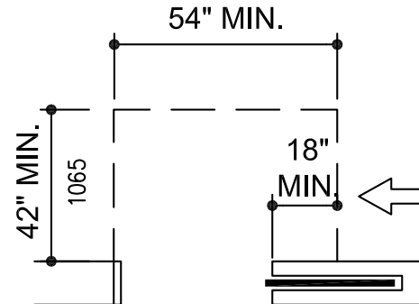
SLIDE SIDE APPROACH
