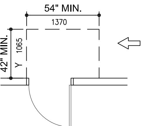
HINGE-SIDE APPROACHES - SWINGING DOORS
