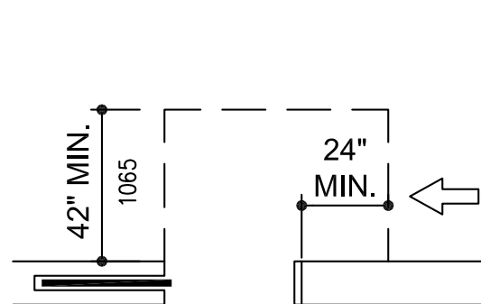
LATCH SIDE APPROACH
