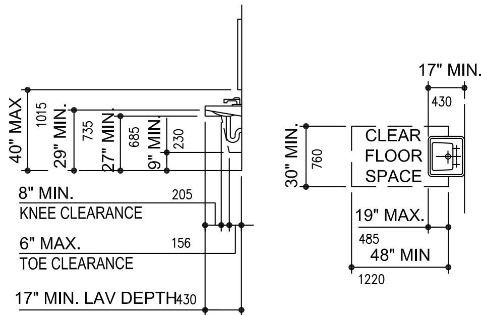
CLEAR FLOOR SPACE AT LAVATORIES
