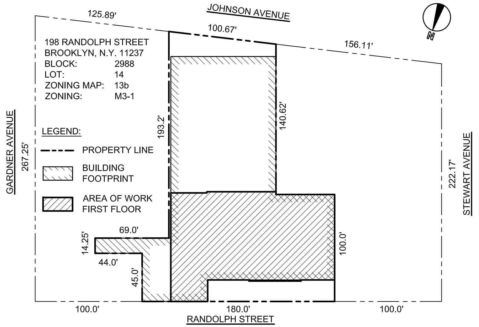
PLOT PLAN
